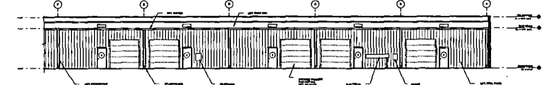
4 REAR ELEVATION
