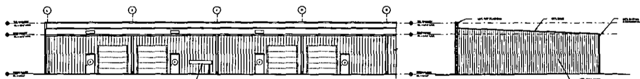
5 REAR ELEVATION
